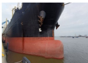
Vsl Outside Shell F - Overview
